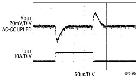
Dual Phase Single Output Load Transient Response, 5\text{V}_{\text{IN}} to 1\text{V}_{\text{OUT}}
