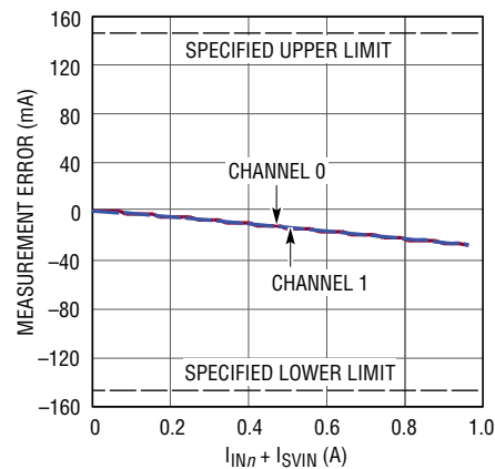
MFR_READ_IIN n (Input Current Readback) Error vs (I_{\text{VIN}n} + I_{\text{SVIN}}) , \text{MFR\_PWM\_MODE}_n[0] = 1_b , I_{\text{OUT}n} Swept from 0\text{A} to 9\text{A} , One Channel at a Time, \text{RUN}_{1-n} = 0\text{V}
