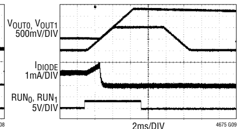
Dual Output Start-Up/Shutdown with a Pre-Biased Load
