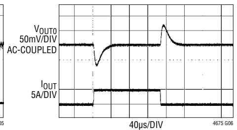
Single Phase Single Output Load Transient Response, 12\text{V}_{\text{IN}} to 1\text{V}_{\text{OUT}}
