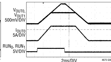
Dual Output Concurrent Rail Start-Up/Shutdown
