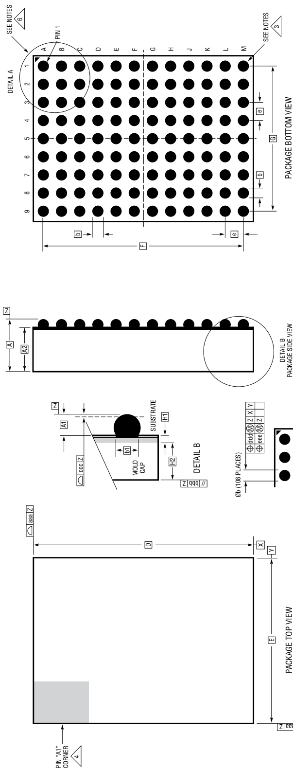
BGA Package 108-Lead (16mm × 11.9mm × 3.51mm) (Reference LTC DWG # 05-08-1931 Rev B)
