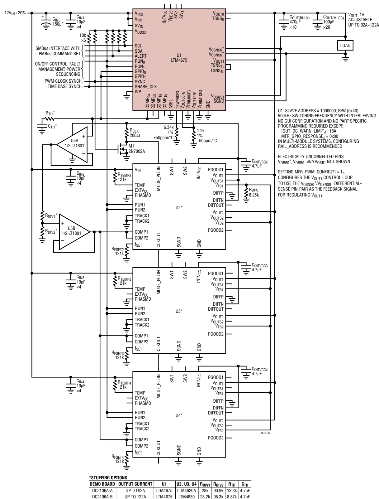
Figure 32. One LTM4675 Operating In Parallel with 3xLTM4620A or 3xLTM4630 (See Demo Boards DC2106A-A, DC2106A-B, Custom-Stuffed with LTM4675 Modules for U1) Producing 1V OUT at up to 92A ~ 122A. Power System Management Features Accessible Through LTM4675. See Figure 33
