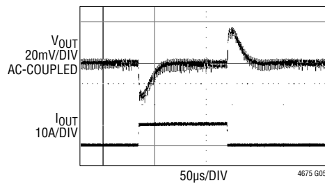
Dual Phase Single Output Load Transient Response, 12\text{V}_{\text{IN}} to 1\text{V}_{\text{OUT}}
