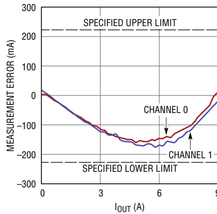
READ_IOUT n (Output Current Readback) Error vs I_{\text{OUT}n}
