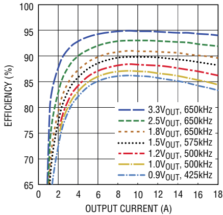
Efficiency vs Load Current at 5\text{V}_{\text{IN}}
