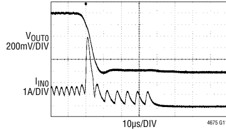
FIGURE 61 CIRCUIT AT 12\text{V}_{\text{IN}} . 112\text{m}\Omega LOAD ON V_{\text{OUT}0} PRIOR TO APPLICATION OF SHORT CIRCUIT
